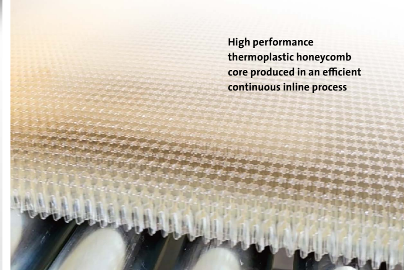
Thermoplastic PEI/CF composite skins on a PEI honeycomb core resulting in a recyclable mono-thermoplastic sandwich material
